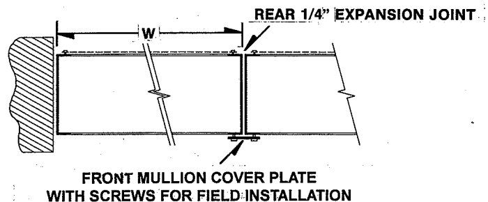
TYPICAL HORIZONTAL SECTION FOR MULTIPLE PANELS
